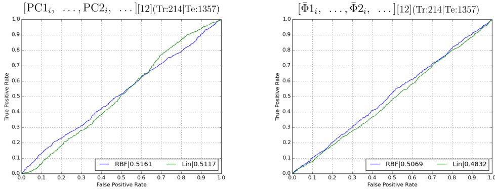
Figure 4.18: ROC plots of the twelve separate oriented components of the phase congruency magnitudes and mean phase angles (i.e. concatenation of outputs of six orientations from two images).
