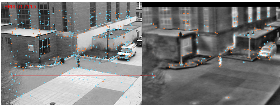
(c) BRISK (1 correct of 113 declared).
